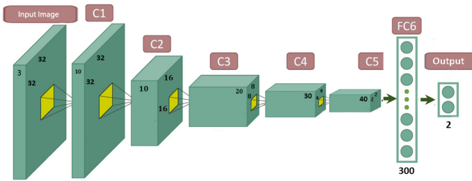
Fig. 6: Model architectures of Corner Refiner. All kernels are 5x5 and applied with padding. ReLU activation is applied after every Convolutional Layer. Two outputs are interpreted as co-ordinates of corner point.
