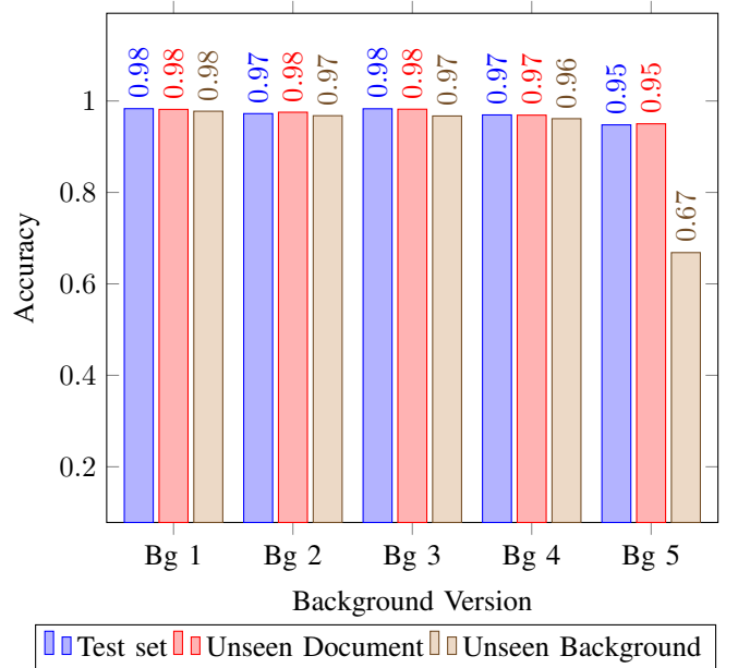
Fig. 8: Experiment 2 and 3 results. System shows good generalization on unseen simple backgrounds and unseen document type
