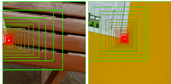
Fig. 4: Recursive Corner Refinement. Based on prediction the area least likely to contain the point is discarded and cropped image is fed to the model again. The squares represent the area that the model sees in each iteration.
