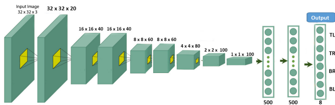
Fig. 3: Model architecture for corner detection. 5 \times 5 kernels are used and Rectified Linear Unit (ReLU) is applied after every convolutional layer. The eight outputs are interpreted as co-ordinates of four corners.
